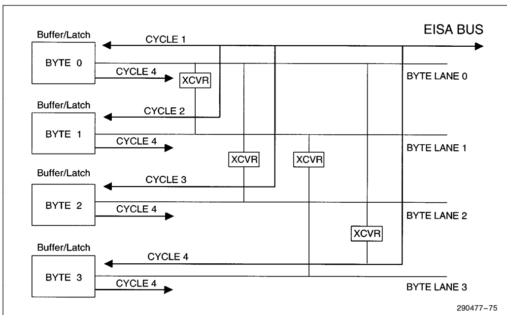
Figure 31. Re-Drive Function: 32-bit EISA Master Accessing an 8-bit EISA or ISA Slave 32-bit Read—BE[3:0] # = 0000
