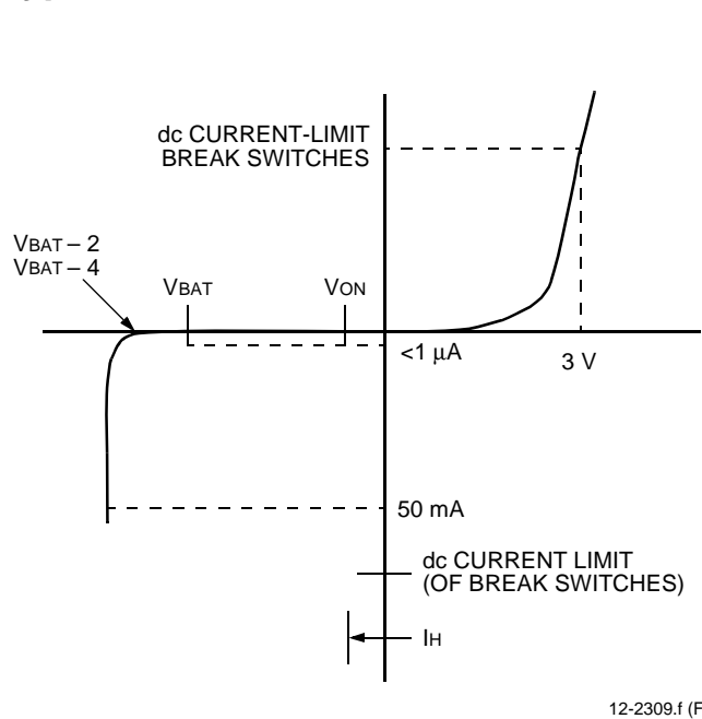
Figure 3. Protection Circuit A Version
