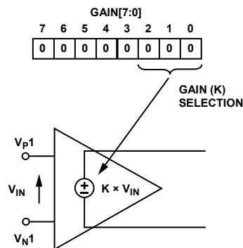
Figure 30. PGA in Current Channel
