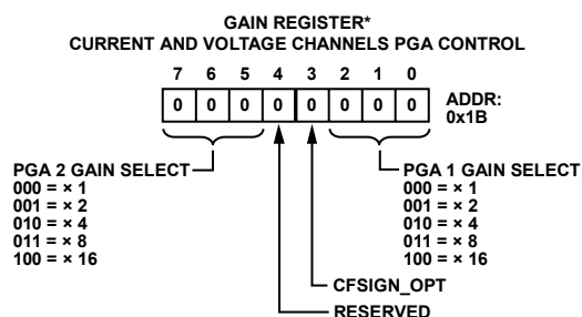
Figure 30. PGA in Current Channel
