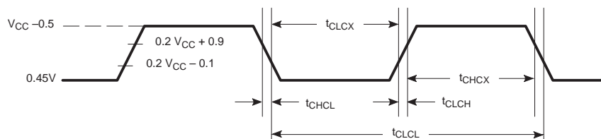
Figure 1. External Clock Drive
