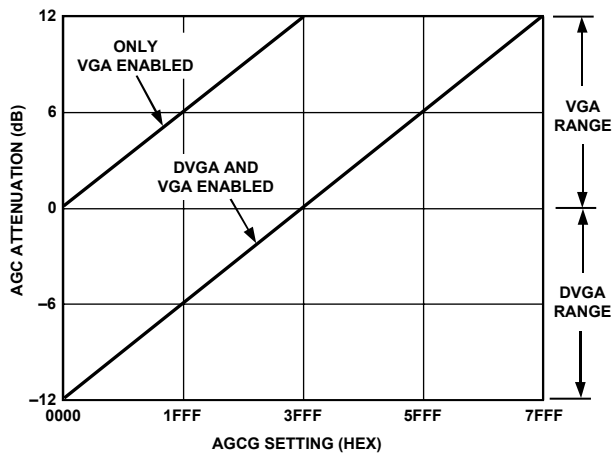
Figure 59. AGC Gain Range Characteristics vs. AGCG Register Setting with and without DVGA Enabled
