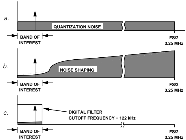
Figure 12. Sigma-Delta ADC
