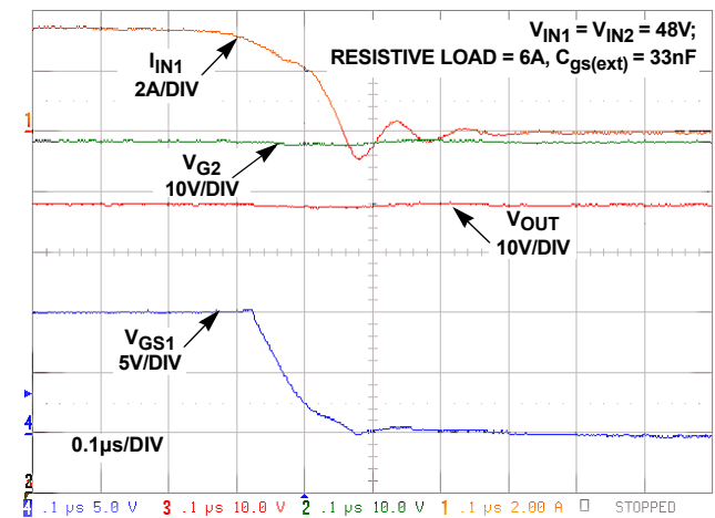
FIGURE 23. FAST SPEED TURN-OFF (MOSFET WITH Q_{TOT} = 8.4nC ) AND 33nF EXTERNAL C_{\text{GS}}
