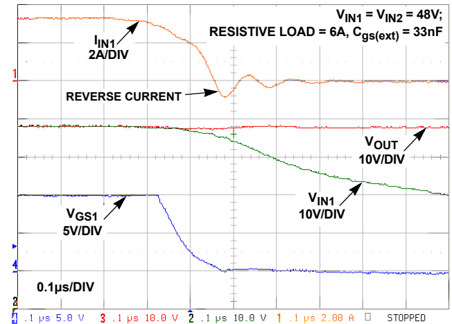
FIGURE 22. FAST SPEED TURN-OFF (MOSFET WITH Q_{TOT} = 8.4nC ) AND 33nF EXTERNAL C_{\text{GS}}
