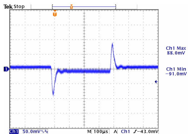
Figure 13. Vin=12V, Vout=1.8V
