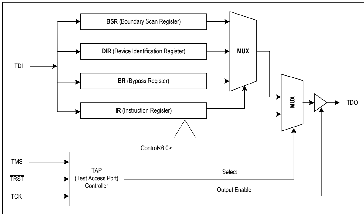
Figure 40. JTAG Architecture
