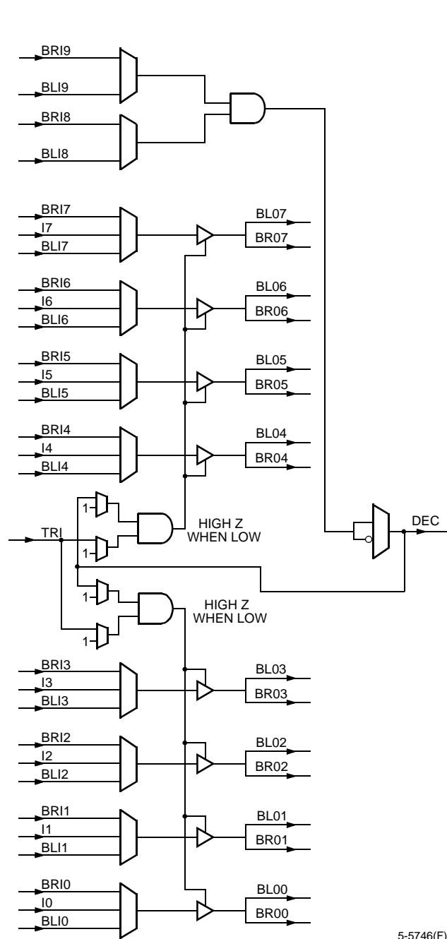
Figure 13. Buffer-Buffer-Decoder Mode
