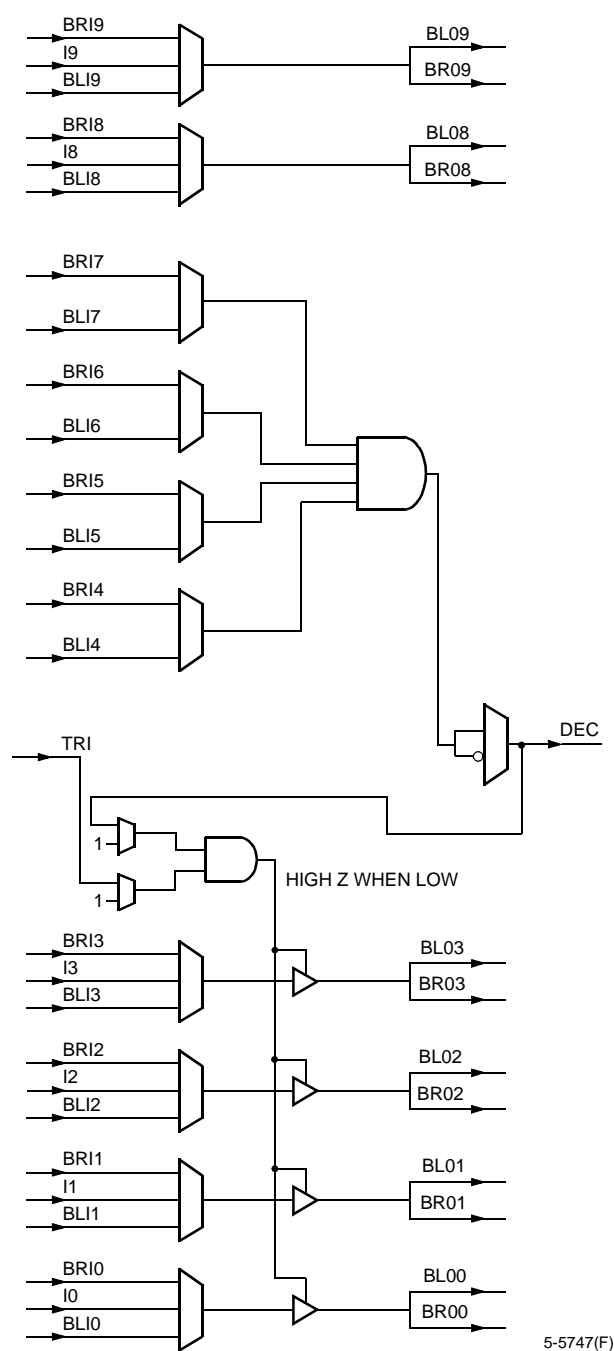
Figure 14. Buffer-Decoder-Buffer Mode
