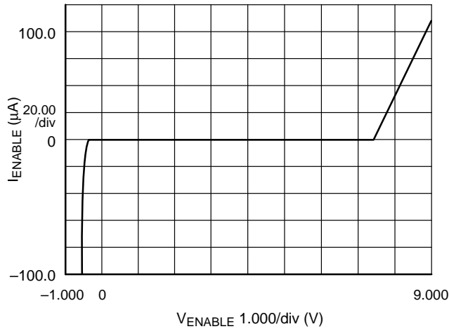
Figure 10. \overline{\text{ENABLE}} Input Current vs. Input Voltage
