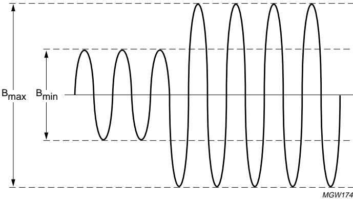
Fig.3 Definition of modulation index.
