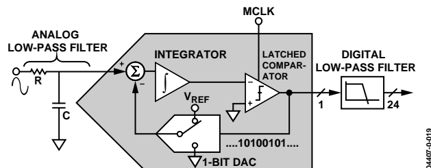
Figure 17. First-Order \Sigma\text{-}\Delta ADC
