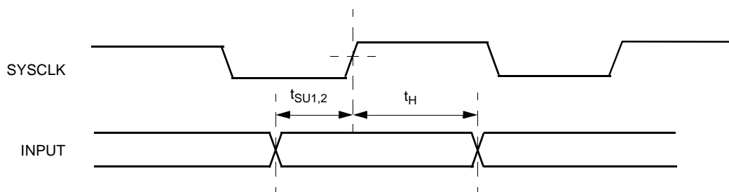
Figure 7-5. Input Timing
