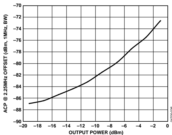
Figure 36. Adjacent Channel Power vs. Output Power, CDMA2000 Single Carrier @ 1960 MHz; ACP Measured at \pm 2.25 MHz Carrier Offset (1 MHz BW); V_{BB1} = V_{BBQ} = 0.353 V
