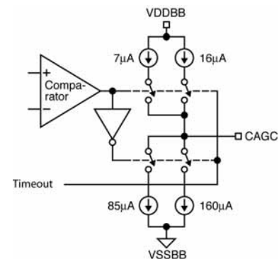
Figure 3. CAGC Pin
