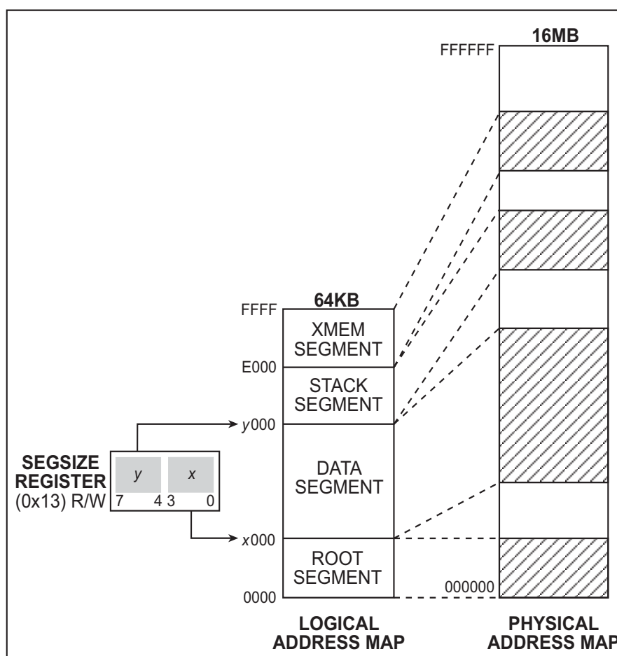
Figure 5-2. Logical and Physical Memory Mapping
