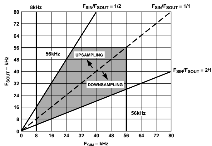
Figure 11. Allowable Input and Output Sample Frequencies F_{CRYSTAL} = 16 \text{ MHz} Case
