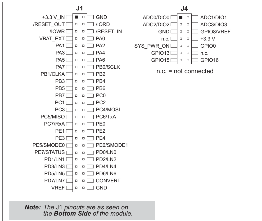
Figure 7. RCM4510W Pinout
