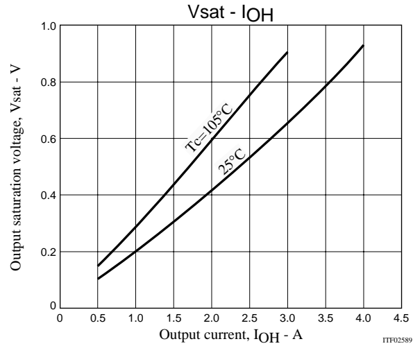
STK672-740B-E Output saturation voltage, V_{sat} - Output current, I_{OH}
