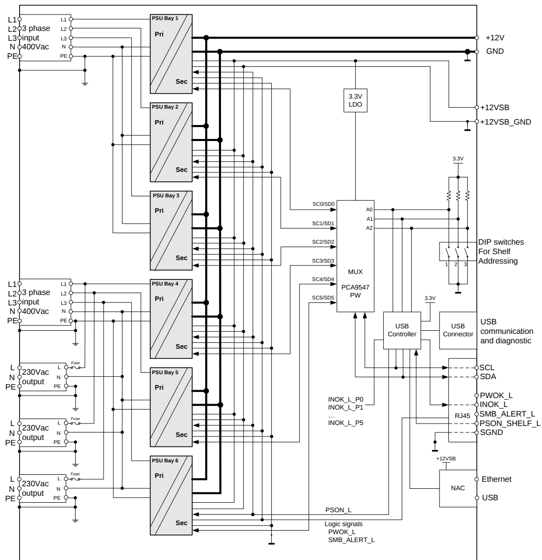
Figure 1. SPSPF3-0XG Block Diagram
