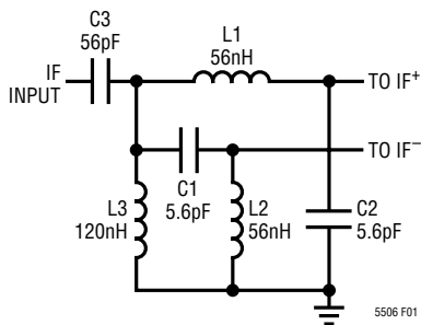
Figure 1. IF Input Matching Network at 280MHz
