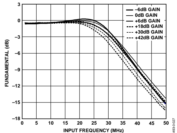
Figure 72. Effects of RxPGA Gain on LPF Frequency Response ( f_{-3\text{dB}} = 32\text{ MHz} @ 0 dB and f_{\text{ADC}} = 80\text{ MSPS} )
