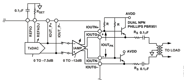
Figure 65. Voltage-Mode Operation
