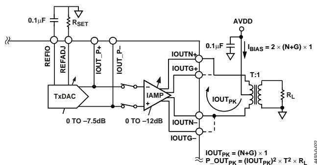
Figure 64. Current-Mode Operation
