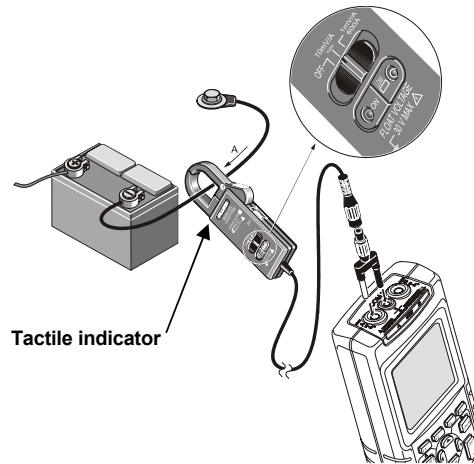
Figure 2. Measuring Setup.
