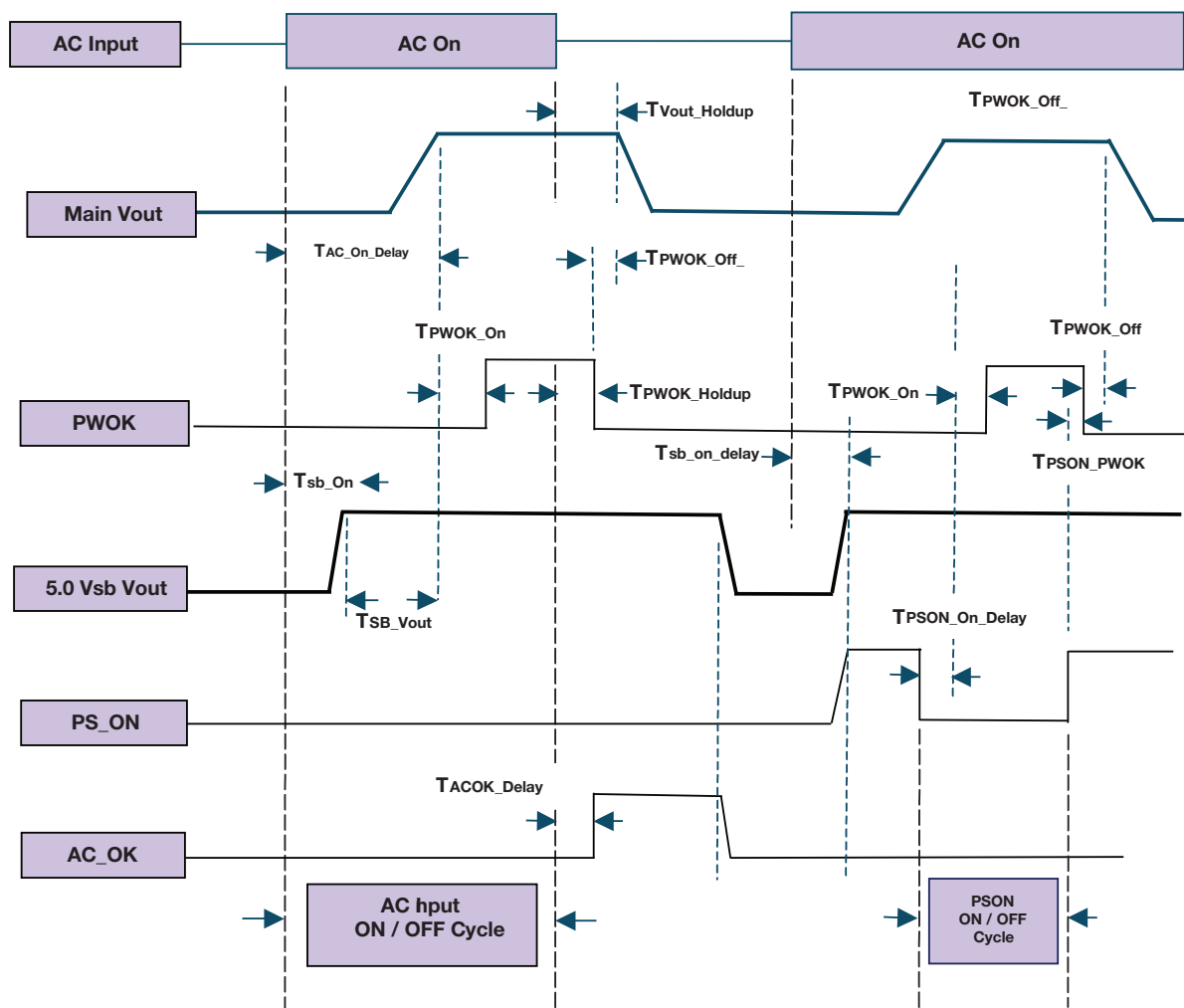
Timing Diagram
