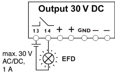
Figure 9 EFD ground fault monitoring
