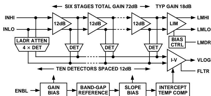
Figure 25. Main Features of the AD8309
