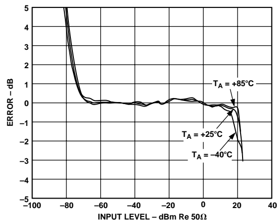
Figure 10. Log Linearity of RSSI Output vs. Input Level, 100 MHz Sine Input, at T_A = -40^\circ\text{C} , +25^\circ\text{C} , and +85^\circ\text{C}
