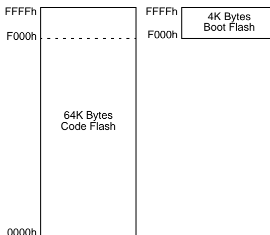
Figure 7-1. Program/Code Memory Organization
