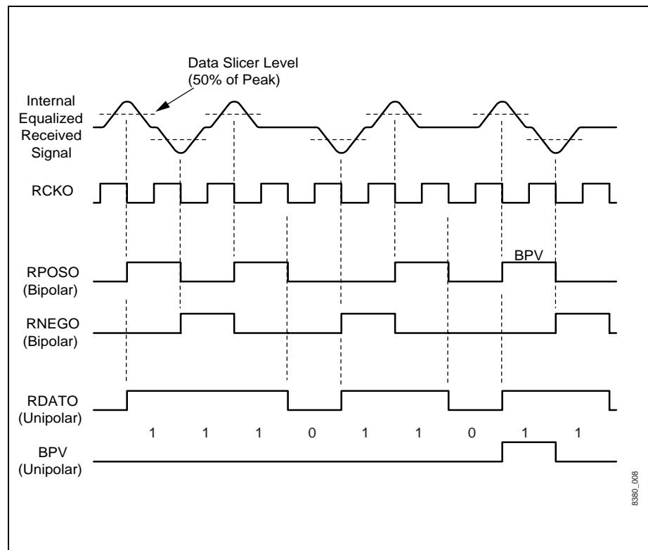
Figure 2-3. Receiver Signals
