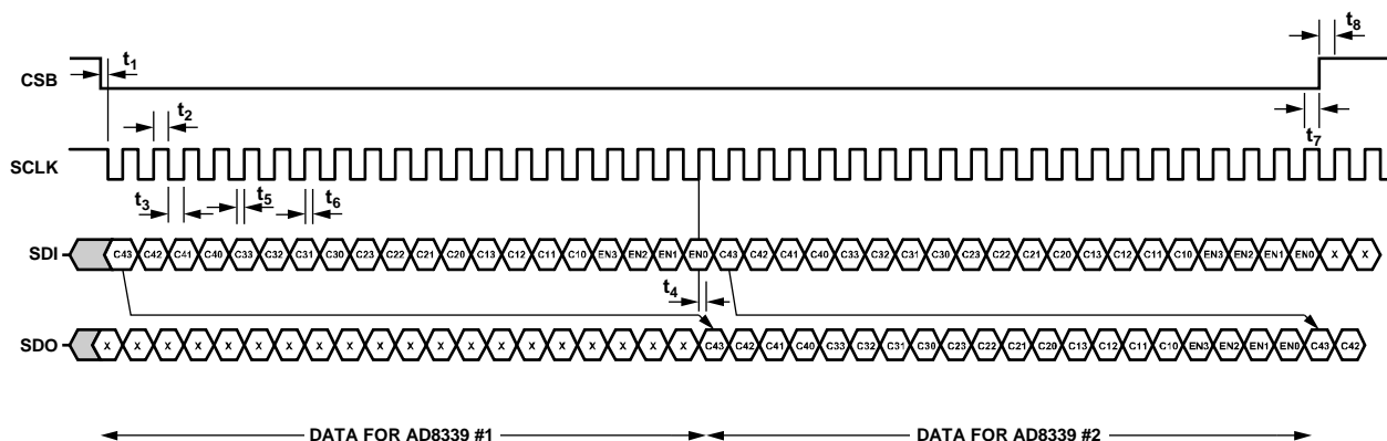
Figure 57. Timing Diagram
