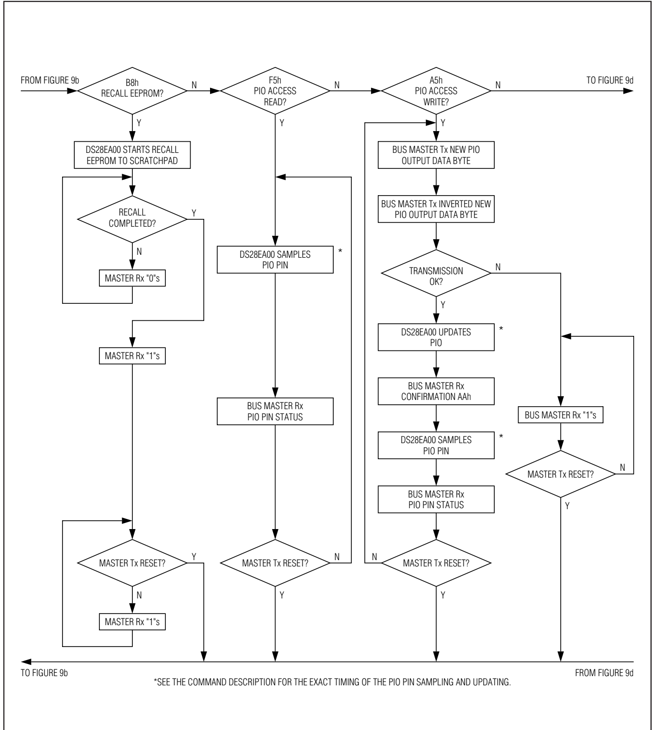
Figure 9c. Control Function Flowchart
