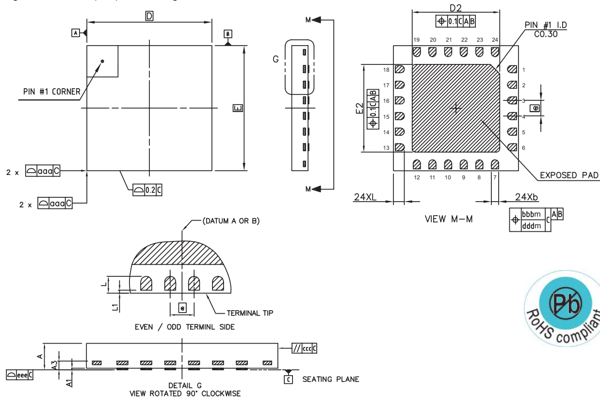
Figure 28. TQFN(4x4)-24 Package
