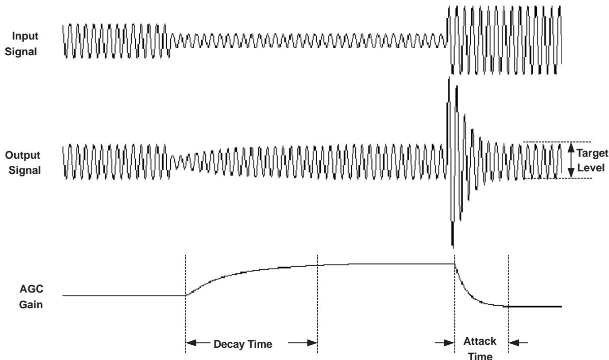
Figure 28. Typical Operation of the AGC Algorithm During Speech Recording
