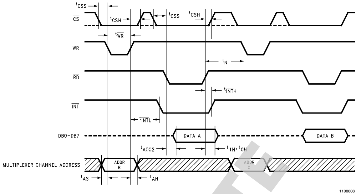
FIGURE 3. \overline{WR} - \overline{RD} Mode (Mode Pin is High and t_{RD} > t_{INTL} )
