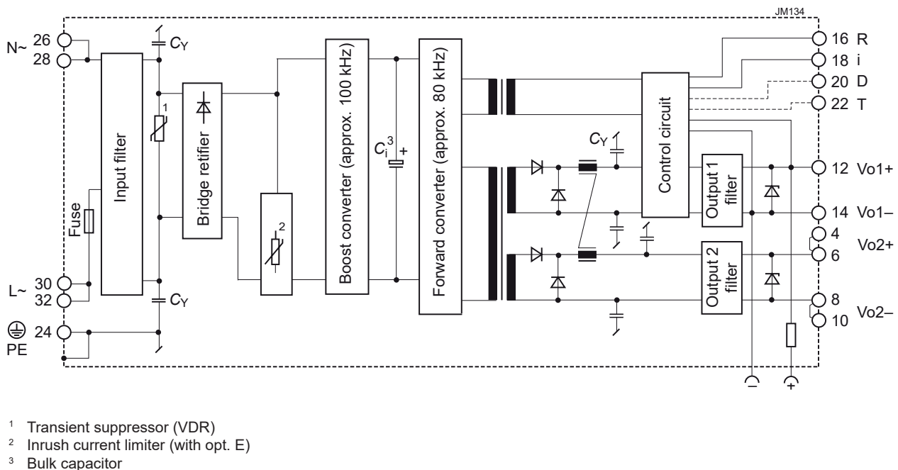
Fig. 1 Block diagram of a converter
