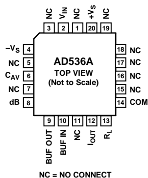
Figure 5. E-20 Package Pin Configuration
