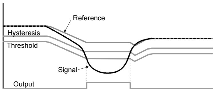
Figure 1-7 Drift Compensation
