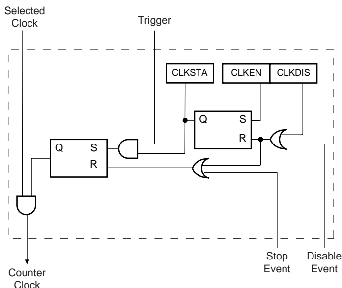
Figure 140. Clock Control
