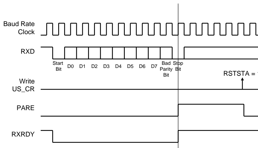
Figure 100. Parity Error
