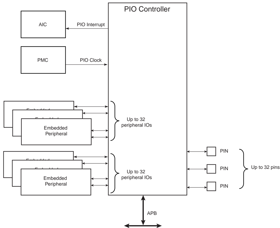
Figure 65. Block Diagram
