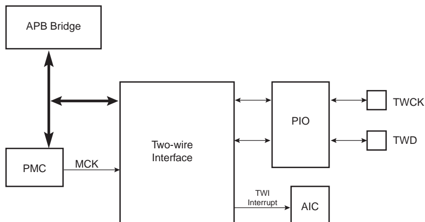
Figure 79. Block Diagram
