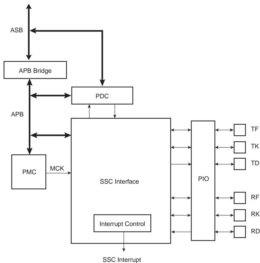
Figure 120. Block Diagram
