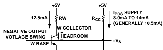
Figure 14. Negative Swing
