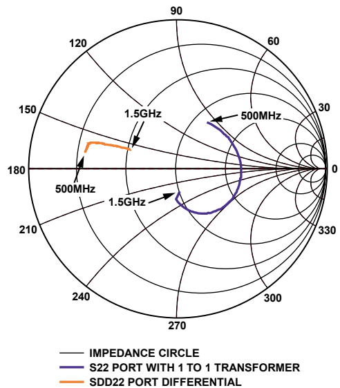
Figure 21. Output Impedance Smith Chart (with Frequency Markers)
