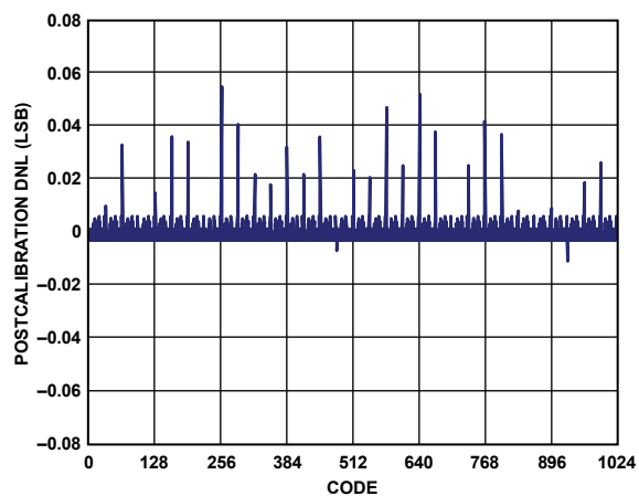
Figure 27. AD9115 Postcalibration DNL at 1.8 V, 8 mA
