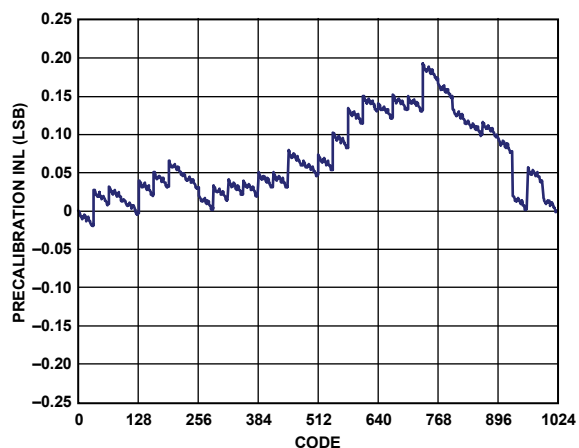
Figure 25. AD9115 Precalibration INL at 3.3 V, 20 mA
