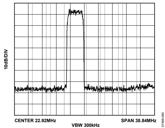
Figure 67. AD9117 ACLR 1-Carrier 3.3 V
