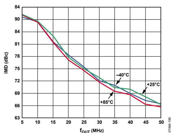
Figure 57. IMD Over Temperature at 8 mA, 3.3 V
