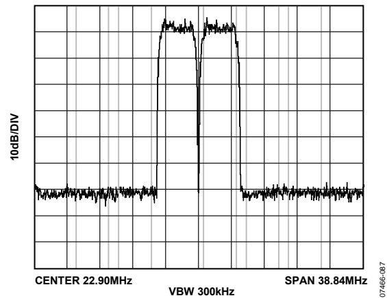
Figure 69. AD9117 ACLR 2-Carrier 3.3 V
