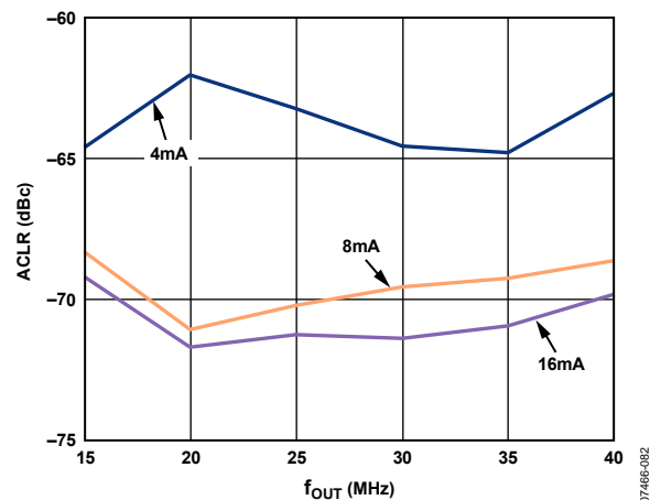
Figure 51. AD9117 2-Carrier W-CDMA Second Adjacent Channel ACLR 3.3 V
