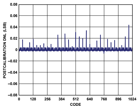
Figure 29. AD9115 Postcalibration DNL at 3.3 V, 20 mA
