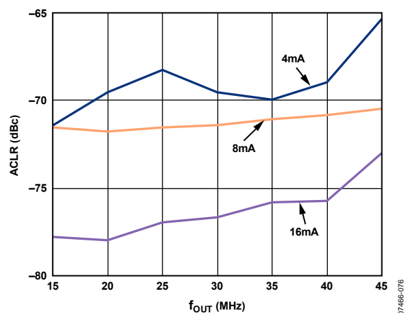
Figure 45. AD9117 1-Carrier W-CDMA Second Adjacent Channel ACLR 3.3 V
