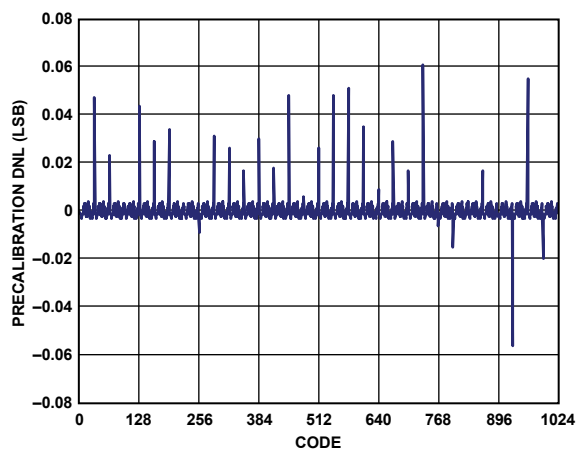
Figure 26. AD9115 Precalibration DNL at 3.3 V, 20 mA
