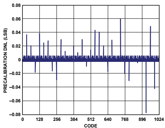
Figure 24. AD9115 Precalibration DNL at 1.8 V, 8 mA
