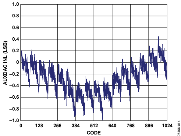
Figure 37. AUXDAC INL
