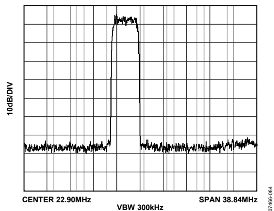
Figure 66. AD9117 ACLR 1-Carrier 1.8 V
