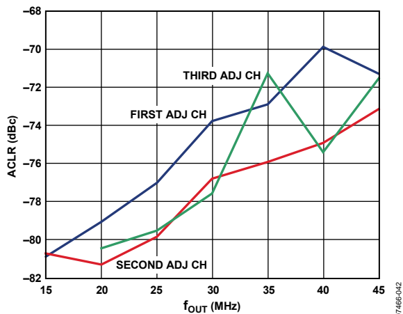
Figure 38. AD9117 Close In ACLR at 3.3 V, 20 mA
