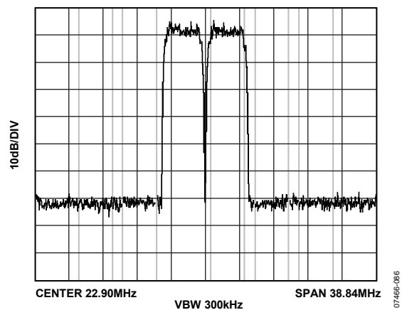
Figure 68. AD9117 ACLR 2-Carrier 1.8 V
