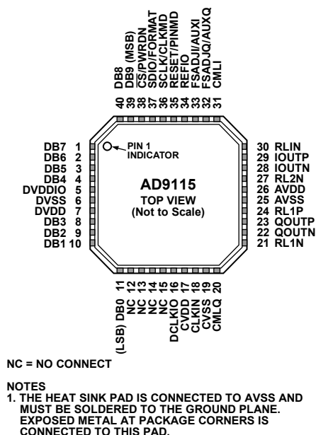
Figure 4. AD9115 Pin Configuration
