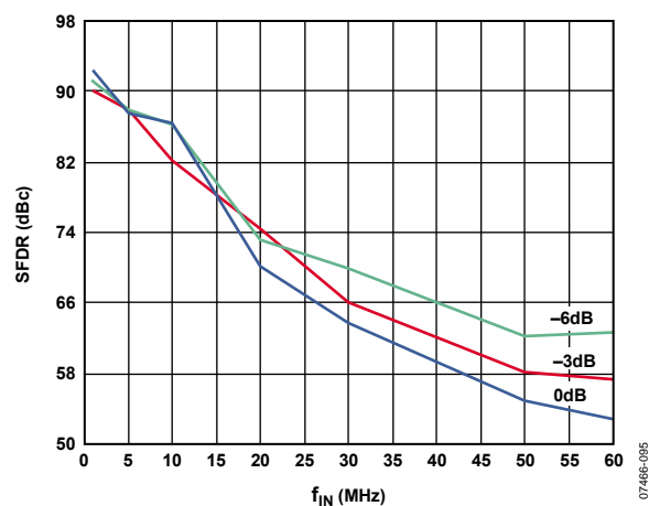
Figure 59. SFDR vs. Digital Signal Level 3.3 V
