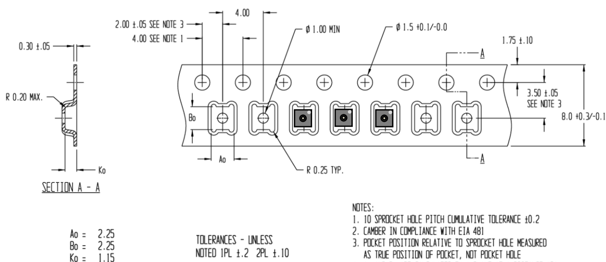
Figure 12 Technical drawing of the packaging tape with sensor orientation in tape. Header tape is to the right and trailer tape to the left on this drawing. Dimensions are given in millimeters.
