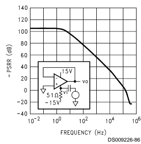
Negative Power Supply Voltage Rejection Ratio
