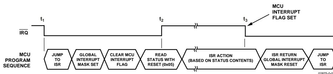
Figure 45. ADE7753 Interrupt Management
