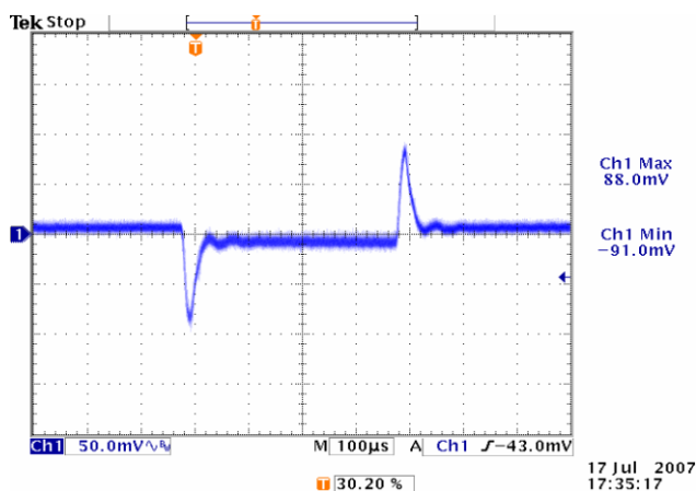
Figure 13. Vin=12V, Vout=1.8V
