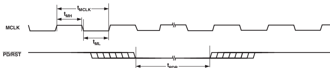
Figure 1. MCLK and \overline{\text{PD}}/\overline{\text{RST}} Timing
