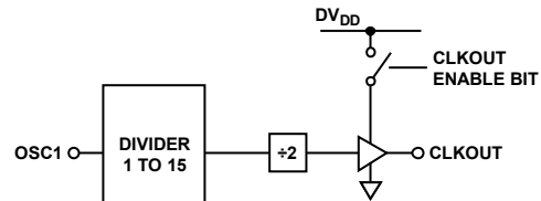
Figure 32. CLKOUT Stage
