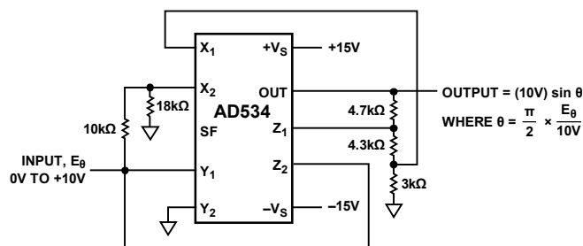
Figure 21. Voltage-Controlled Amplifier
