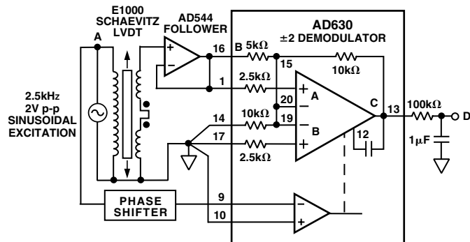
Figure 11. LVDT Signal Conditioner
