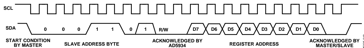
Figure 25. Timing Diagram
